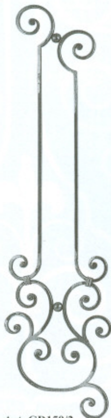
Art. GD159/2 Mtl 9/16" x 5/16" 11 1/32" W x 39 3/8" H Wt. 6.2 lbs.
