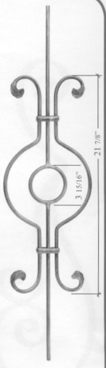
Art. 1074/2 Mtl 3/8" dia. 9 1/16" W x 39 1/2" H Wt. 4.0 lbs.
