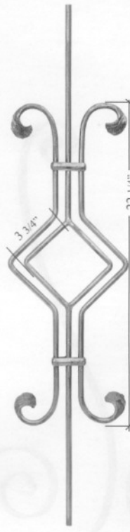
Art. 1074/1 Mtl 3/8" dia. 8 1/16" W x 39 1/2" H Wt. 4.1 lbs.
