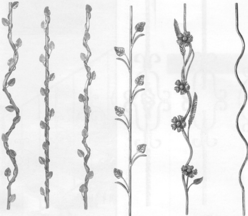
Art. 604/6 Mtl 1/2" dia. 39 1/2"H Wt. 4 lbs. Art. 604/7 Mtl 1/2" dia. 39 1/2"H Wt. 3 lbs. Art. 604/8 Mtl 1/2" dia. 39 1/2"H Wt. 3 lbs. Art. 1170/1 Mtl 1/2" dia. 5 1/8" W x 39 1/2"H Wt. 3.3 lbs. Art. 1171/1 Mtl 1/2" dia. 4 3/4" W x 39 1/2"H Wt. 4.4 lbs. Art. 1171/2 Mtl 1/2" dia. 2 3/8" W x 39 1/2"H Wt. 2.2 lbs.
