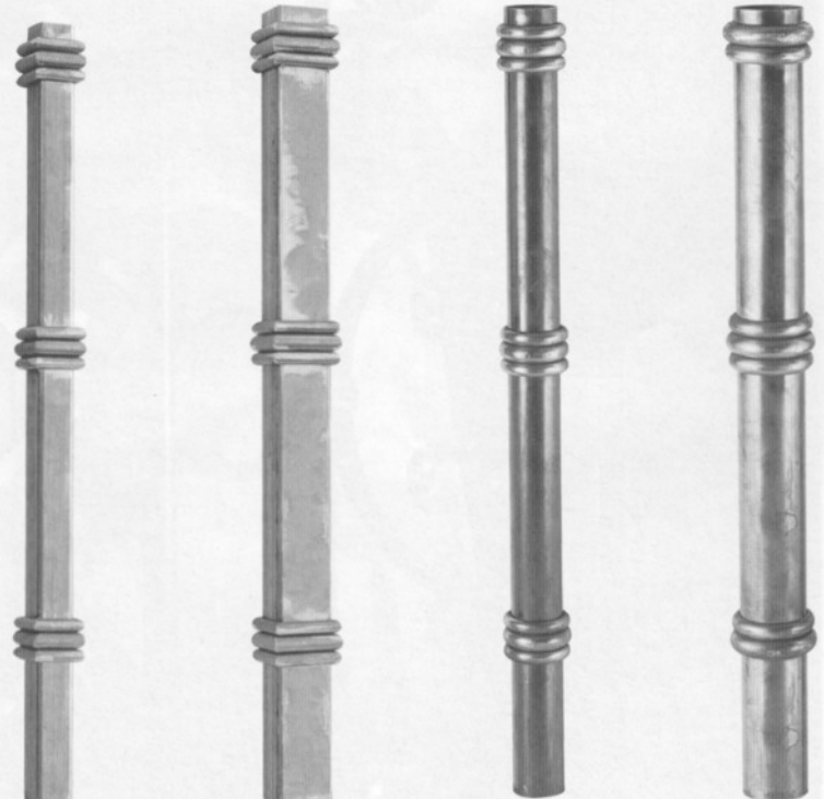
Art. 1207/1 Mtl 2 3/8" sq. 3 11/32" W x 47 1/4" H Wt. 26.4 lbs. Art. 1207/2 Mtl 3 5/32" sq. 4 1/8" W x 47 1/4" H Wt. 33 lbs. Art. 1207/3 Mtl 2 15/16" dia. 3 15/16" W x 47 1/4" H Wt. 24 lbs. Art. 1207/4 Mtl 3 15/16" dia. 5 5/16" W x 47 1/4" H Wt. 29.7 lbs.
