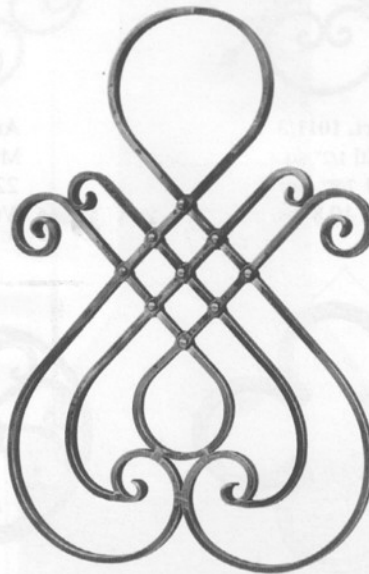
Art. 1657/4 (ex 9104/5) Mtl 5/8" x 5/16" 22 5/8" x 15 3/4" Wt. 8.8 lbs.
