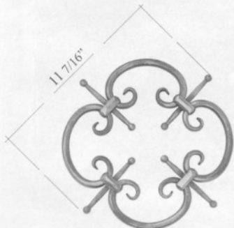
Art. 1014/2 Mtl 1/2" dia. 10 5/8" dia. Wt. 3.3 lbs.
